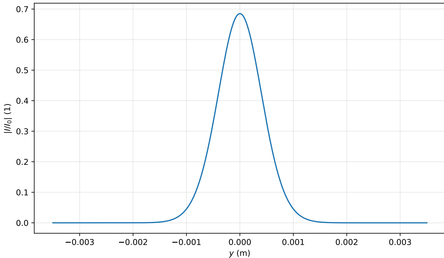
Intensity profile I(x=0, y, z=1.672)/I_0 , P_{in}=0.2P_{cr} , artificial time
